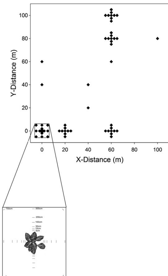
Fig. 1. Diagram showing the layout of seed packets in 100 m × 100 m grids relative to the focal plant and the 500 cm × 500 cm portion of each grid. In the large grid diagram, each diamond indicates the location of a seed packet, while in the close-up seed packet locations are indicated by a dash (–). The close-up shows the focal conspecific plant in the 500 cm × 500 cm portion of each array. Note that seed packet distances from the focal plant in the close-up are not drawn to scale.
